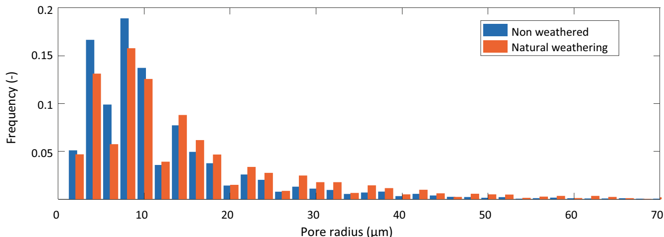
Fig. 7 – Comparison of pore radius distribution of non-weathered marble samples, in blue, and natural weathering, in orange.
