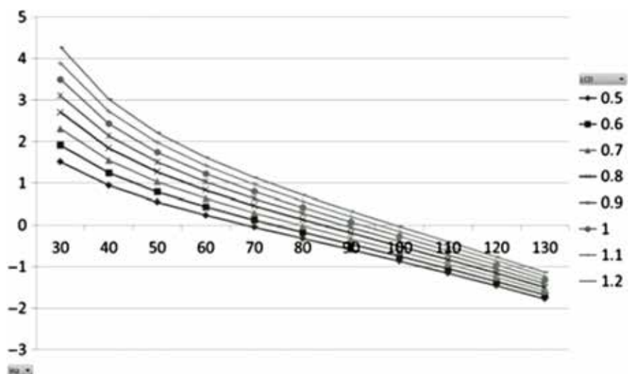
Fig. 4 – Gain of energy [kWh/km] at various speeds [km/h] for different lengths of the charging device [m].
